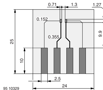
Fig. 4 - Board for R_{\theta JA} Definition (in mm)
