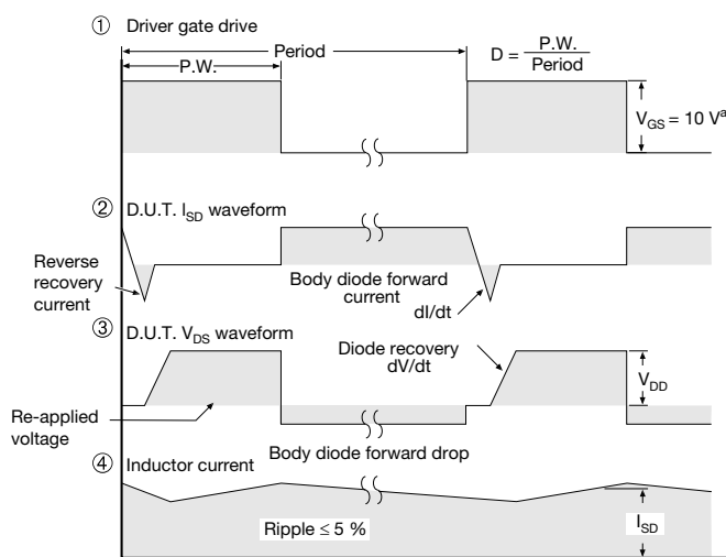
Fig. 20 - For N-Channel
