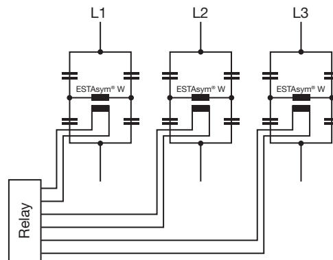
Fig. 2 - Bridge connection
