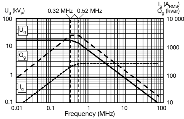
WF125300BH103##BJ1
