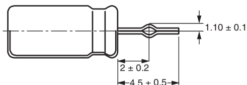
10 \leq \varnothing D \leq 18 leads shortened and formed MALREKL06... (S = 5/7.5 mm)
