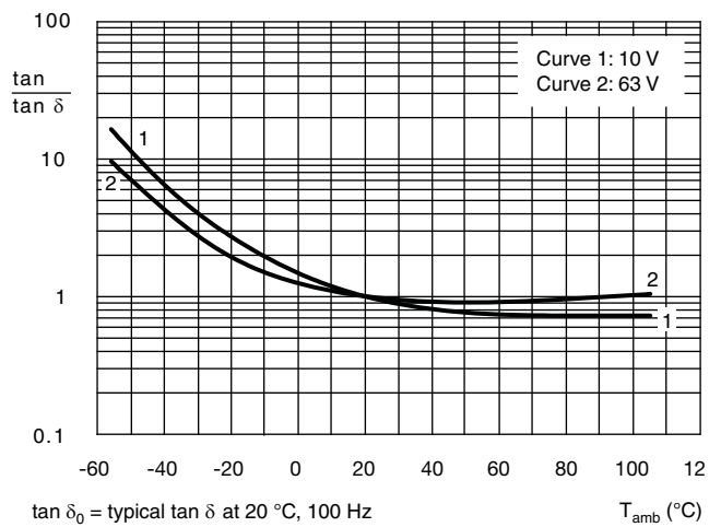
Fig. 6 - Typical multiplier of dissipation factor (tan δ) as a function of ambient temperatures
