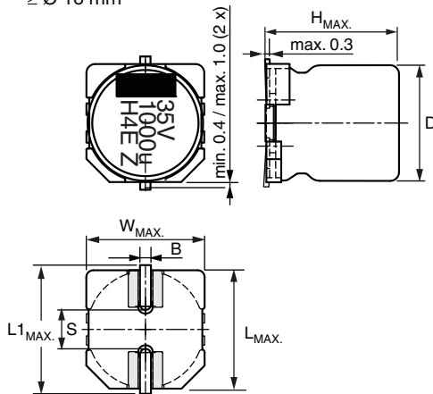
Fig. 2 - Dimensional outline
