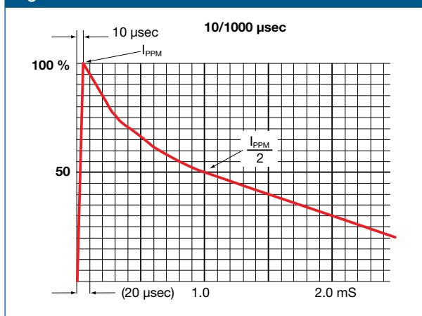
Figure 1. Test waveform of TVS
