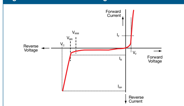
Figure 3. Parameters of voltage and current
