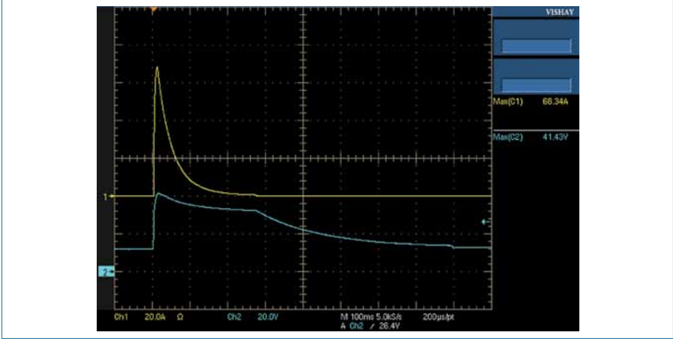
Figure 7a: Clamped voltage and current of SM5S24A in ISO 7637-2 test
