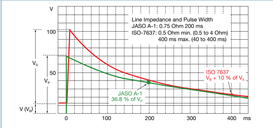
Figure 6. For ISO-7637-2 test conditions, the standard condition is a V_s range of 65 V to 87 V, and R_i (line impedance) range of 0.5 \Omega to 4 \Omega
