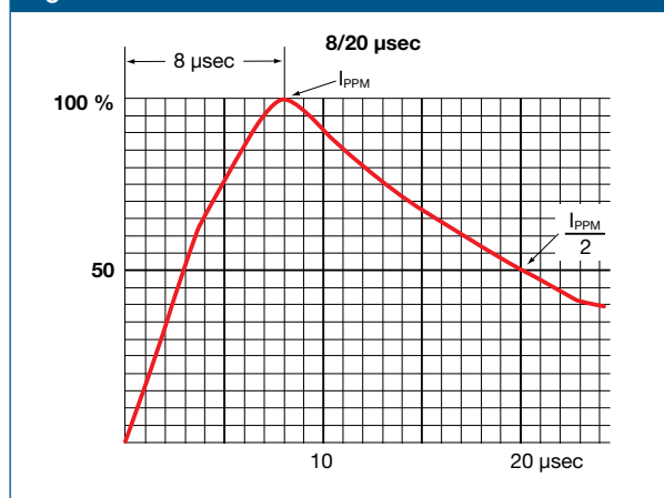
Figure 2. Test waveform of TVS ESD
