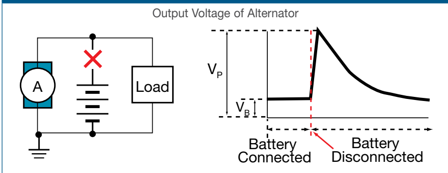
Figure 5. Output voltage of alternator in load dump condition
