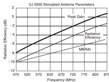
Fig. 1 - Peak Gain and Efficiency vs. Frequency
