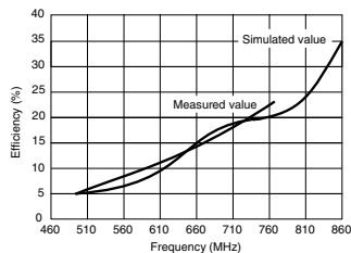
Fig. 2 - Radiation Efficiency vs. Frequency
