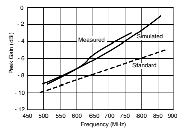
Fig. 1 - Peak gain vs. Frequency
