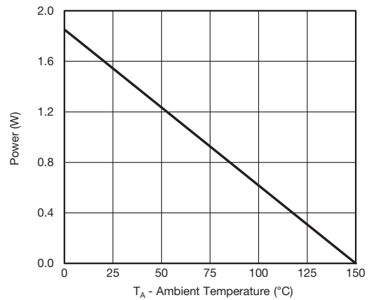
Power, Junction-to-Ambient
