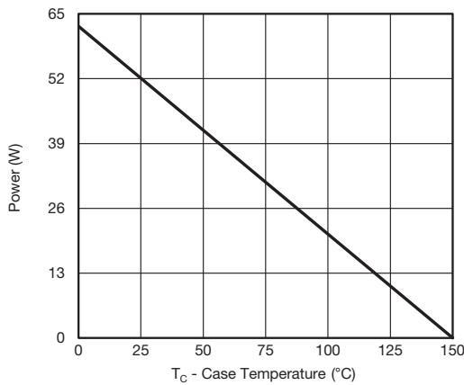
Power, Junction-to-Case
