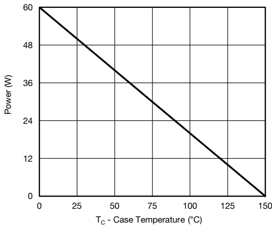
Power, Junction-to-Case
