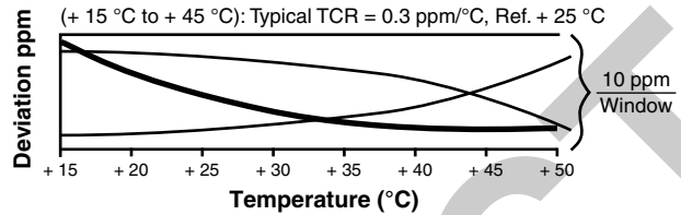
FIGURE 4 - TYPICAL CURVES WITHIN 10 ppm WINDOW, VHP101 LABORATORY INSTRUMENT RANGE
