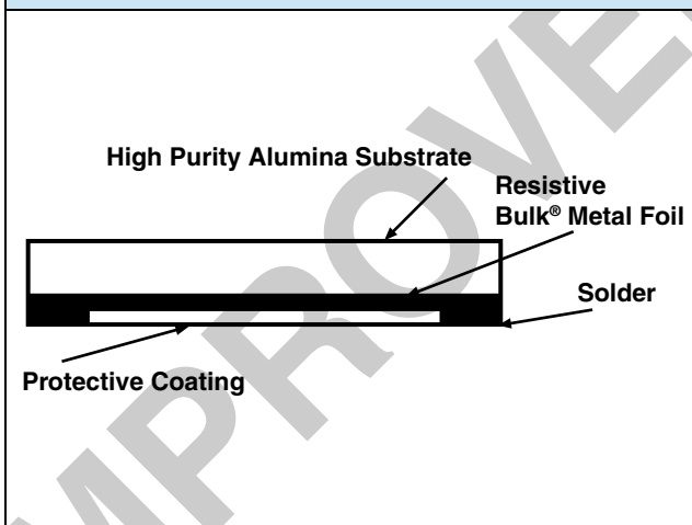
FIGURE 3 - CHIP CONFIGURATION
