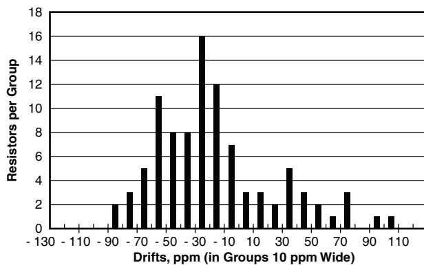
Fig. 3 - Histogram of Drifts for Endurance Testing of 96 Resistors, 10 kΩ, Vishay Style S102C
