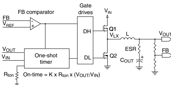
Fig. 2 - On-Time Generation
