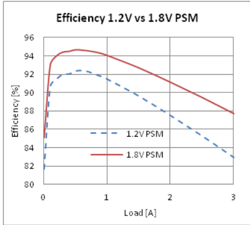
Efficiency vs. I_{OUT} (PSM)
