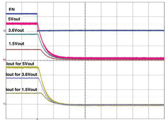
2 V/Div, 0.2 A/Div, 2 \mu s /Div
