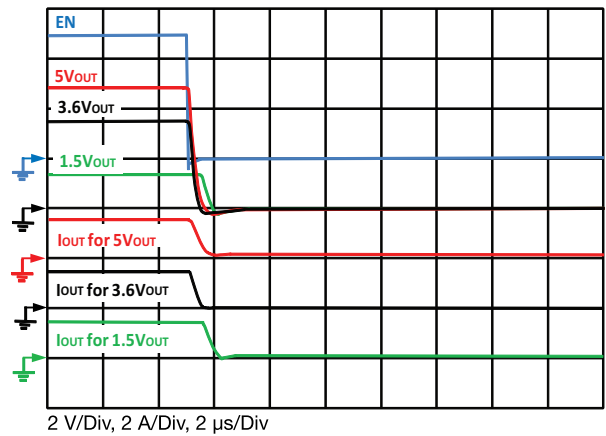
Fig. 21 - Typical Fall Time C_{OUT} = 0.1 \mu F , C_{IN} = 4.7 \mu F , I_{OUT} = 1.5 A
