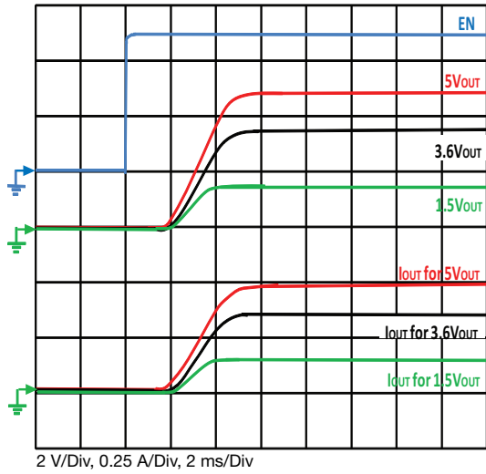
Fig. 24 - Typical Turn-on Delay, Rise Time C_{OUT} = 200 \mu\text{F} , C_{IN} = 4.7 \mu\text{F} , R_{OUT} = 10 \Omega
