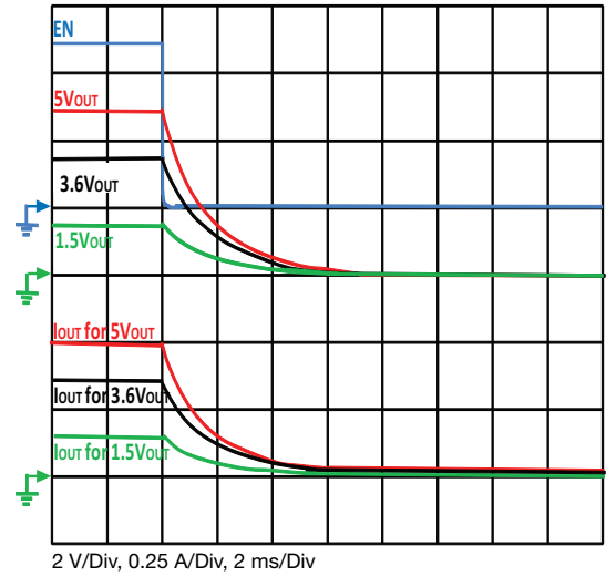
Fig. 25 - Typical Fall Time C_{OUT} = 200 \mu\text{F} , C_{IN} = 4.7 \mu\text{F} , R_{OUT} = 10 \Omega
