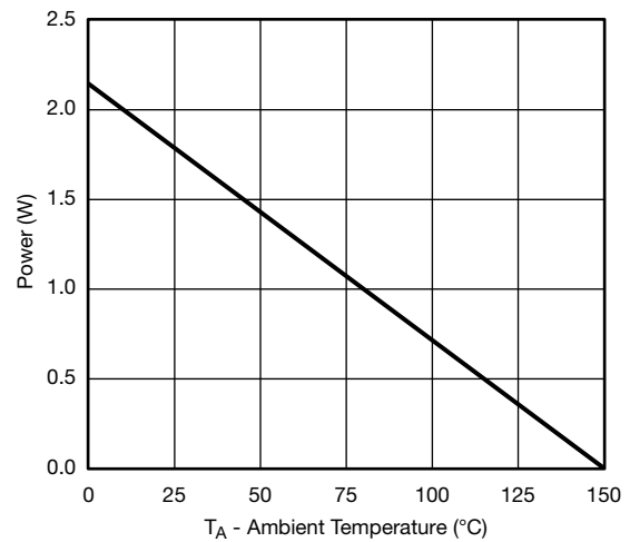
Power, Junction-to-Ambient
