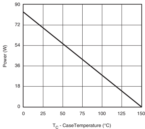
Power, Junction-to-Case
