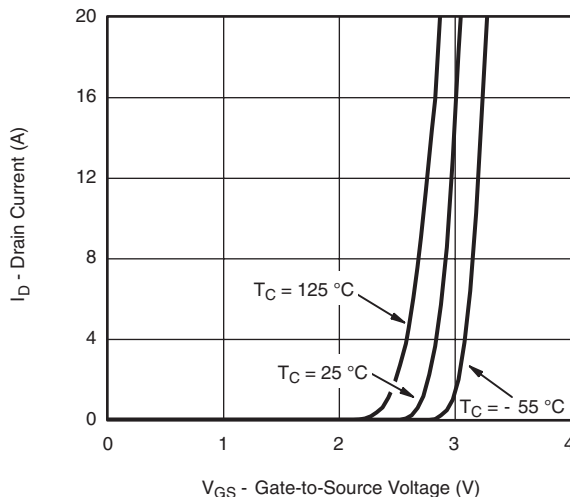
T_C = 125\text{ }^\circ\text{C} T_C = 25\text{ }^\circ\text{C} T_C = -55\text{ }^\circ\text{C} V_{GS} - Gate-to-Source Voltage (V) Transfer Characteristics
