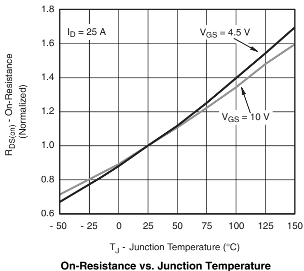
I_D = 25\text{ A} V_{GS} = 4.5\text{ V} V_{GS} = 10\text{ V} R_{DS(on)} - On-Resistance (Normalized) T_J - Junction Temperature ( ^\circ\text{C} ) On-Resistance vs. Junction Temperature
