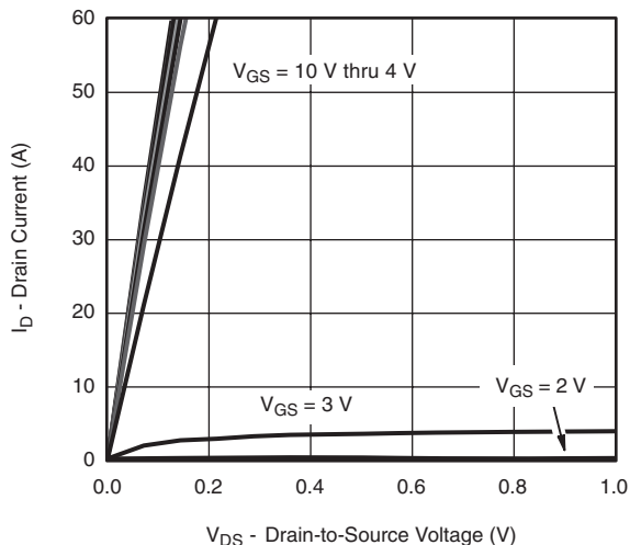
V_{GS} = 10\text{ V thru } 4\text{ V} V_{GS} = 3\text{ V} V_{GS} = 2\text{ V} V_{DS} - Drain-to-Source Voltage (V) Output Characteristics
