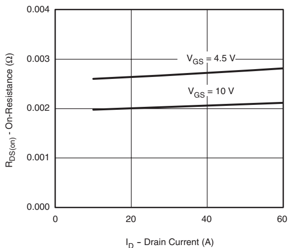
R_{DS(on)} - On-Resistance ( \Omega ) V_{GS} = 4.5\text{ V} V_{GS} = 10\text{ V} I_D - Drain Current (A) On-Resistance vs. Drain Current and Gate Voltage
