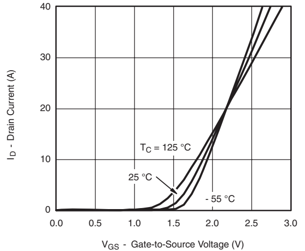
T_C = 125\text{ °C} 25 °C -55 °C Transfer Characteristics
