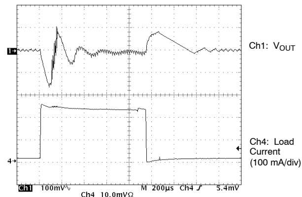
250-mA Transient
