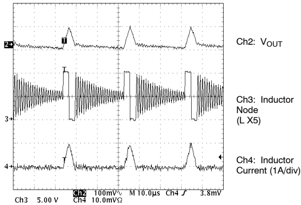
PSM Operation
