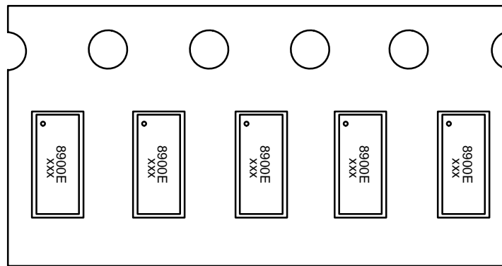
Device on Tape Orientation
