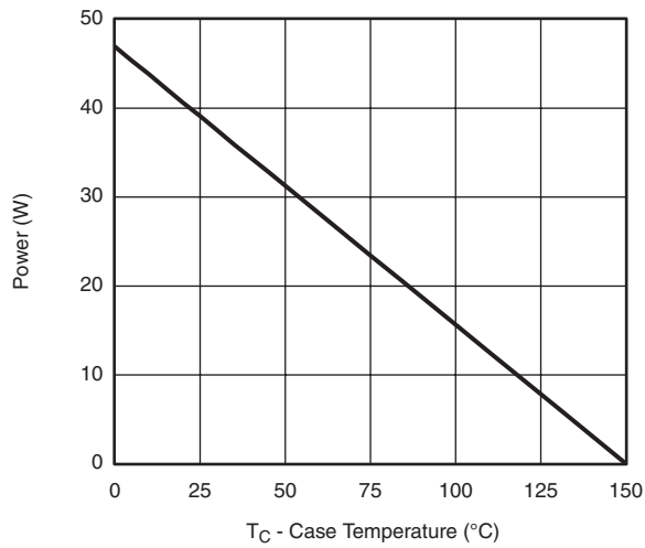
Power Junction-to-Case
