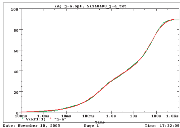
Si5484DU Filter j-a Temperature: 27.0
