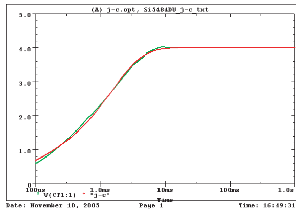
Si5484DU Tank j-c Temperature: 27.0
