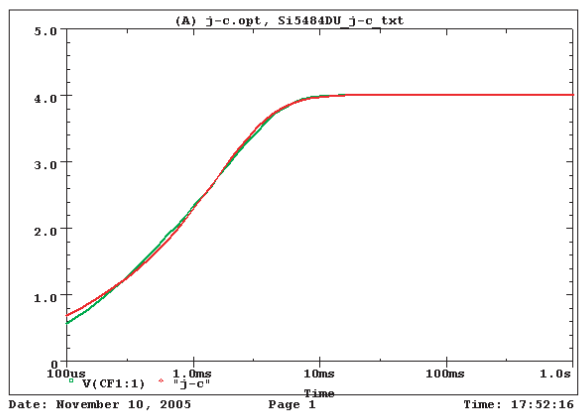
Si5484DU Filter j-c Temperature: 27.0
