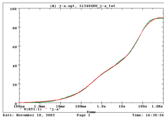
Si5484DU Tank j-a Temperature: 27.0
