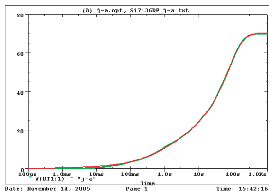
Si7136DP Tank j-a Temperature: 27.0
