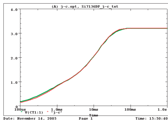
Si7136DP Tank j-c Temperature: 27.0
