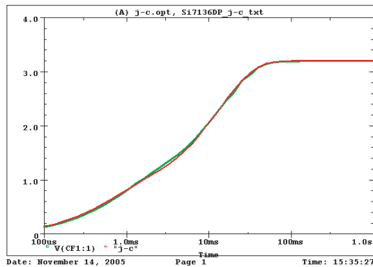
Si7136DP Filter j-c Temperature: 27.0
