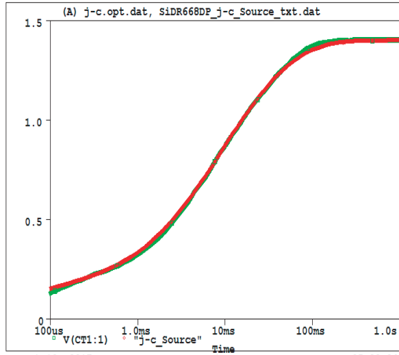
SiDR668DP Tank j-c Source Temperature 27.0
