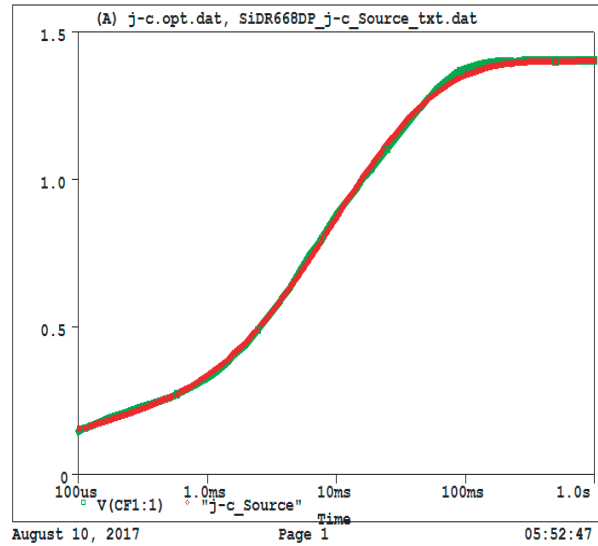
SiDR668DP Filter j-c Source Temperature 27.0
