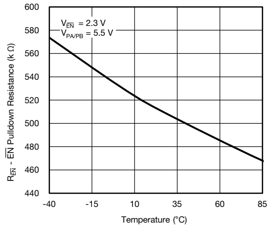
Fig. 9 - EN Pull down Resistance vs. Temperature
