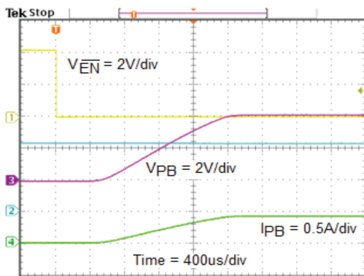
Fig. 17 - Port B Turn-On Time (V PA = 4.2 V, R L = 10 Ω, C L = 0.1 μF)
