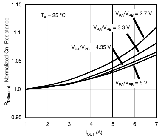
Fig. 10 - Normalized On Resistance vs. Load Current
