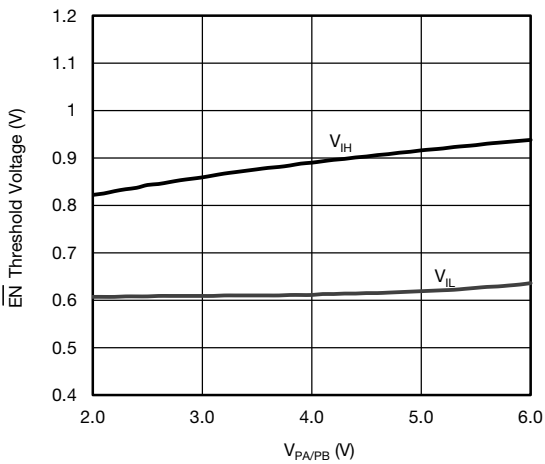
Fig. 13 - \overline{EN} Threshold Voltage vs. Input Voltage
