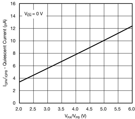
Fig. 3 - Quiescent vs. Input Voltage
