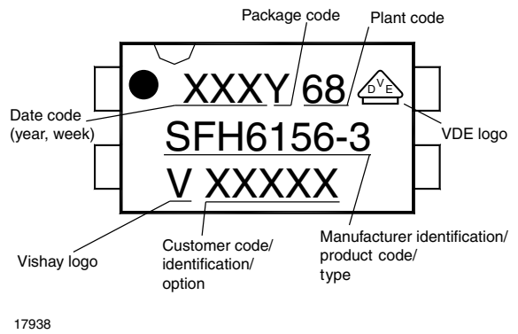
Fig. 5 - DIP-4 Products
