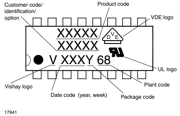
Fig. 9 - DIP-16 Products
