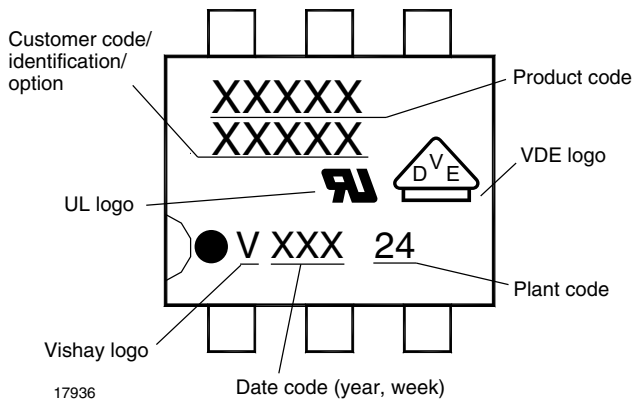
Fig. 3 - DIP-6 Products
