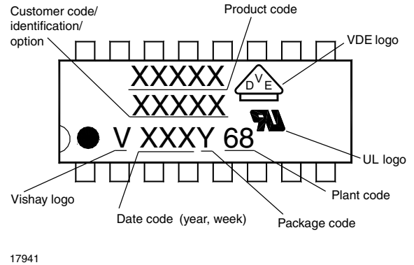
Fig. 9 - DIP-16 Products
