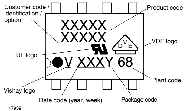
Fig. 6 - DIP-8 Products
