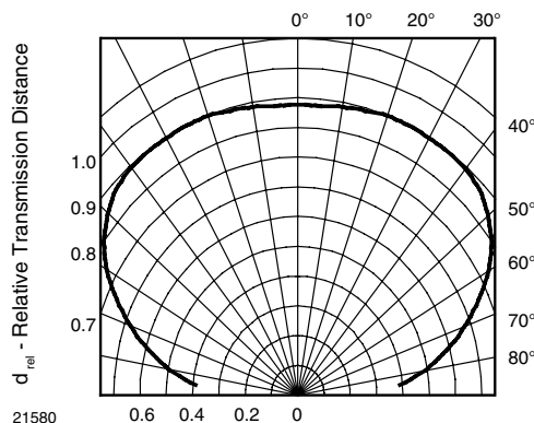
21580 Fig. 13 - Vertical Directivity
