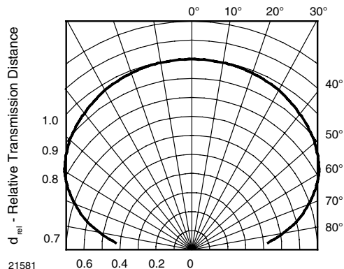
21581 Fig. 12 - Horizontal Directivity
