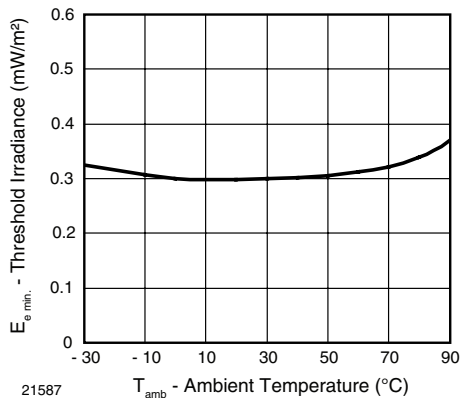
21587 Fig. 10 - Sensitivity vs. Ambient Temperature
