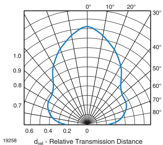
Fig. 11 - Horizontal Directivity
