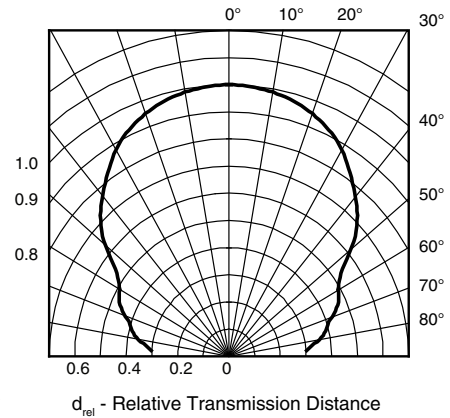
Fig. 12 - Horizontal Directivity
