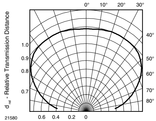
Fig. 13 - Vertical Directivity
