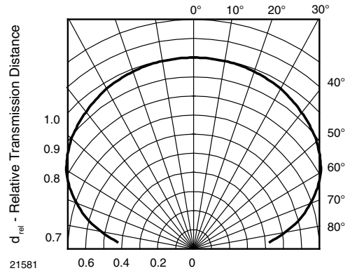
Fig. 12 - Horizontal Directivity
