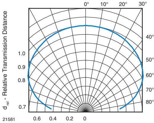
Fig. 11 - Horizontal Directivity
