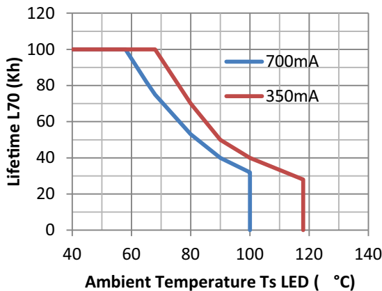
Fig. 5 - Expected Lifetime as a Function of Current and Temperature
