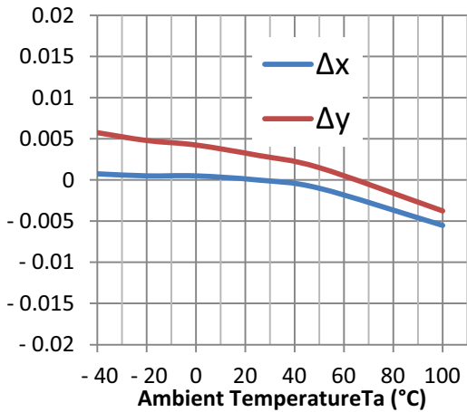
Fig. 4 - \Delta x , \Delta y Color Coordinates Drift vs. Ambient Temperature Measured at 350 mA
