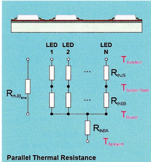
Fig. 7 - Equivalent Circuit Diagram for Thermal Resistance with n LED's on the Board
