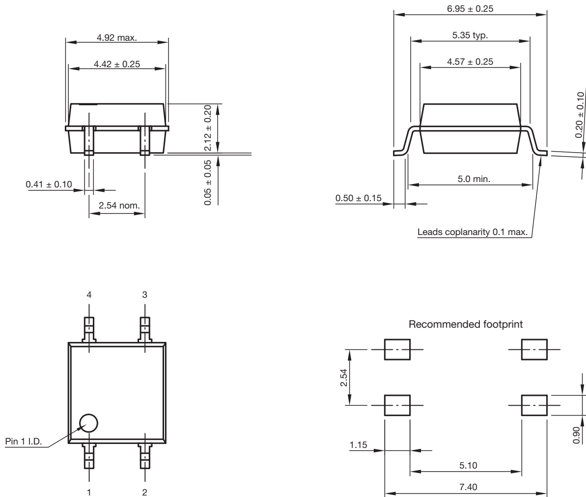
Fig. 15 - Package Drawing
