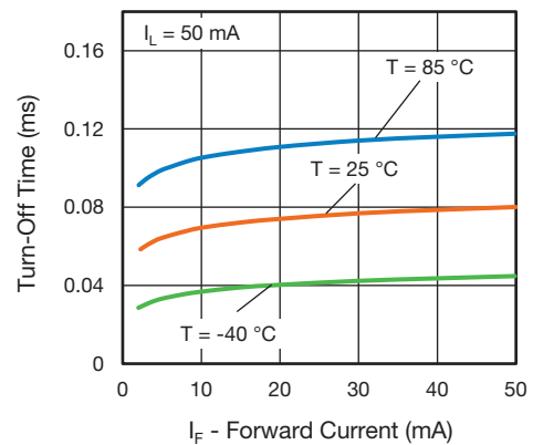
Fig. 13 - Turn-Off Time vs. Forward Current
