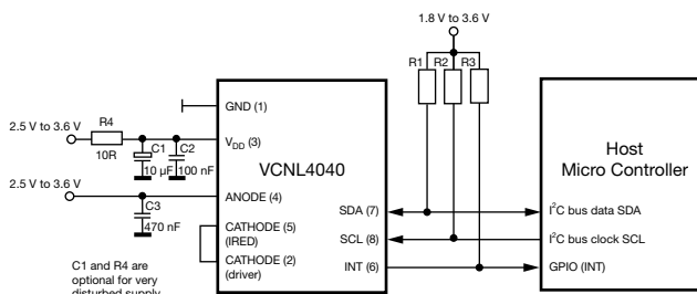
Fig. 5 - VCNL4040 Application Circuit
