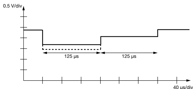
Fig. 13 - Proximity IRED Pulse for 1T
