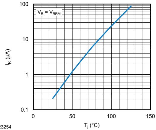
Fig. 3 - Typical Reverse Current vs. Junction Temperature
