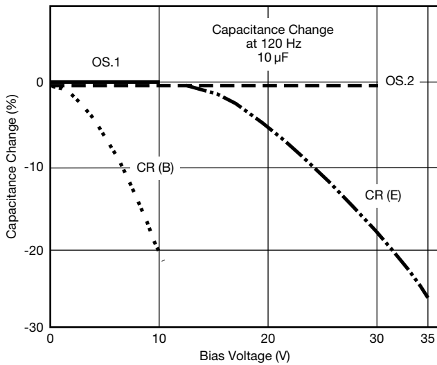
Bias Voltage Characteristics
