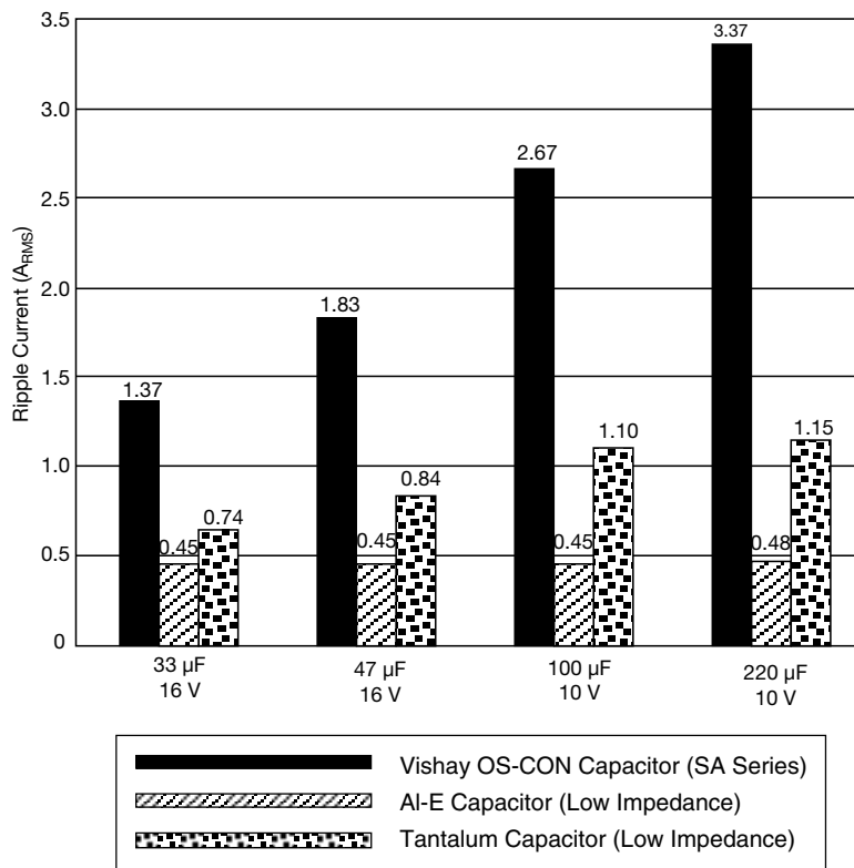
Allowable Ripple Current (100 kHz at + 45 °C)
