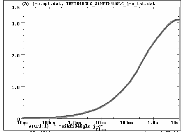
SiHFI840GLC Filter j-c Temperature: 27.0
