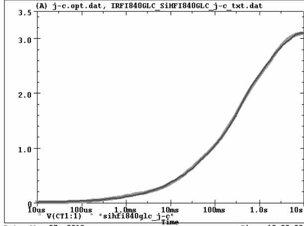
SiHFI840GLC Tank j-c Temperature: 27.0
