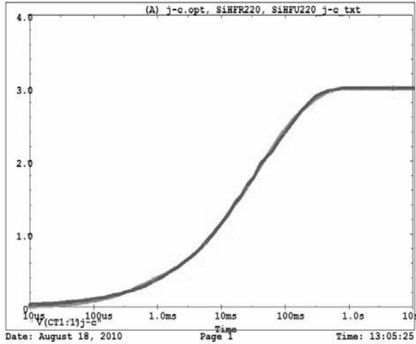
SiHFR220, SiHFU220 Tank j-c Temperature: 27.0
