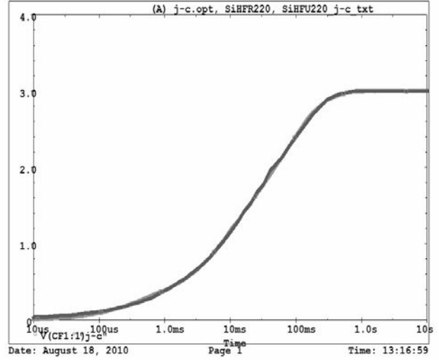
SiHFR220, SiHFU220 Filter j-c Temperature: 27.0
