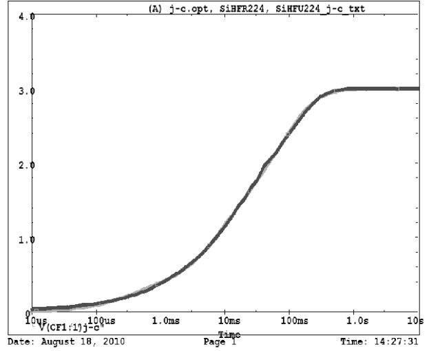
SiHFR224, SiHFU224 Filter j-c Temperature: 27.0
