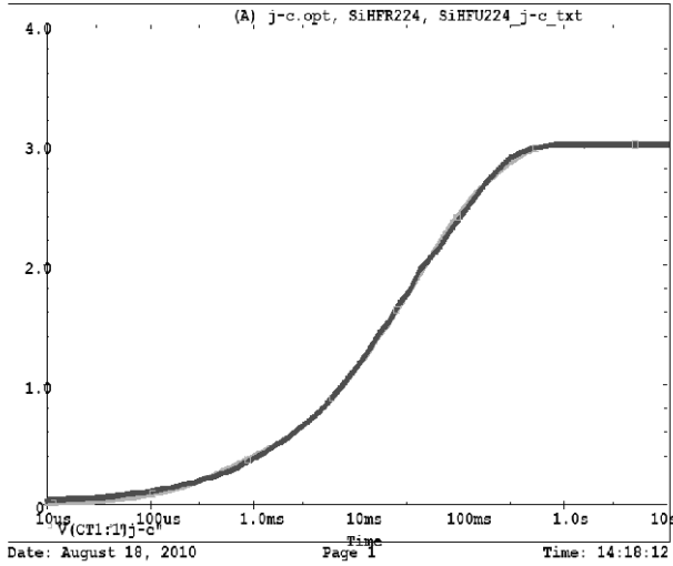
SiHFR224, SiHFU224 Tank j-c Temperature: 27.0
