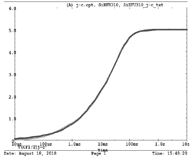
SiHFR310, SiHFU310 Filter j-c Temperature: 27.0
