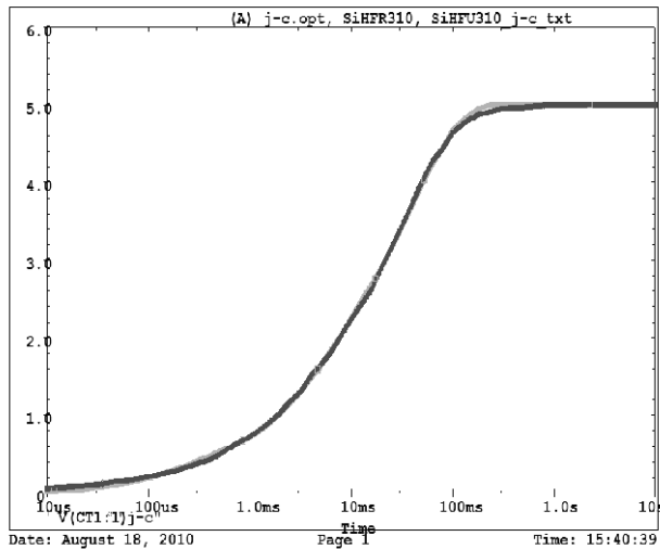
SiHFR310, SiHFU310 Tank j-c Temperature: 27.0
