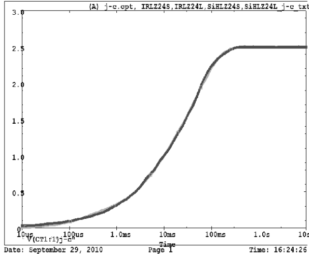
IRLZ24S, IRLZ24L, SiHLZ24S, SiHLZ24L Tank j-c Temperature: 27.0
