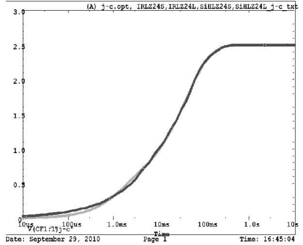
IRLZ24S, IRLZ24L, SiHLZ24S, SiHLZ24L Filter j-c Temperature: 27.0
