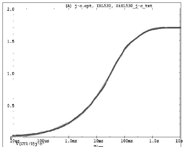
IRL530, SiHL530 Tank j-c Temperature: 27.0
