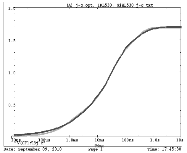
IRL530, SiHL530 Filter j-c Temperature: 27.0
