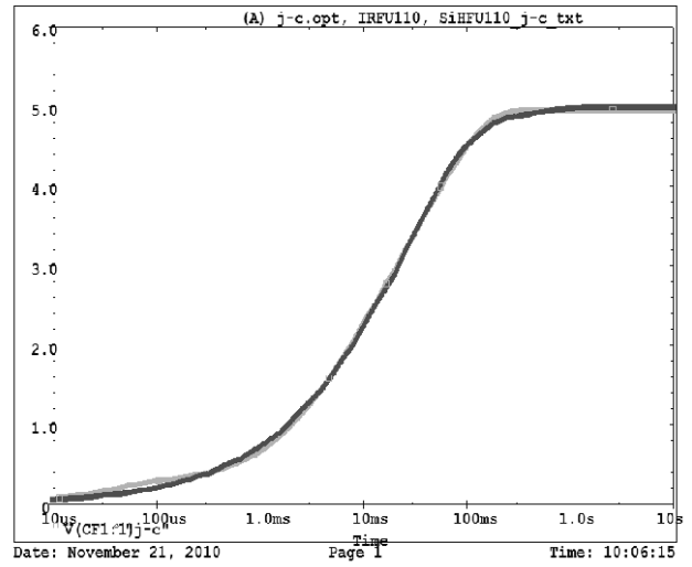
IRFU110, SiHFU110 Filter j-c Temperature: 27.0
