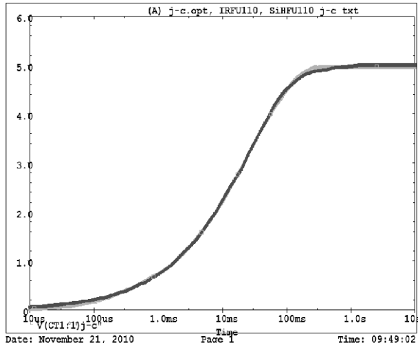
IRFU110, SiHFU110 Tank j-c Temperature: 27.0
