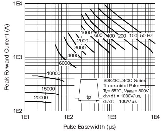
Fig. 33 - Frequency Characteristics
